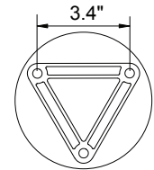
Anchor Bolt M10 x 6.5" (3 anchor bolts and template included)
