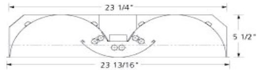
End View: 2 x 2 Recessed Deep Direct/Indirect
